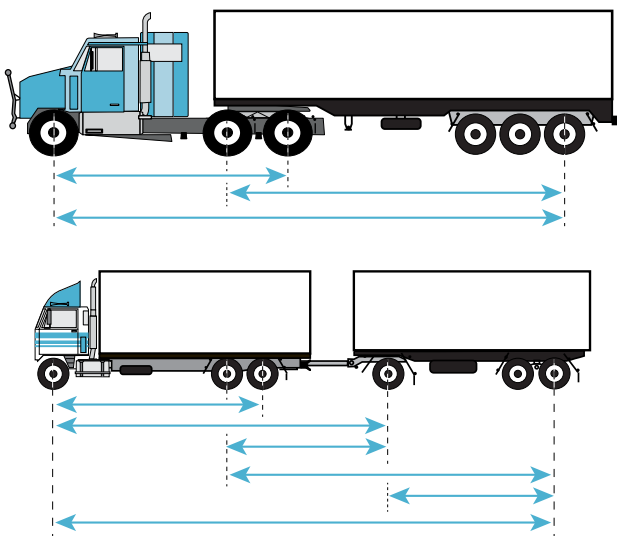
Axle spacings of a heavy vehicle
